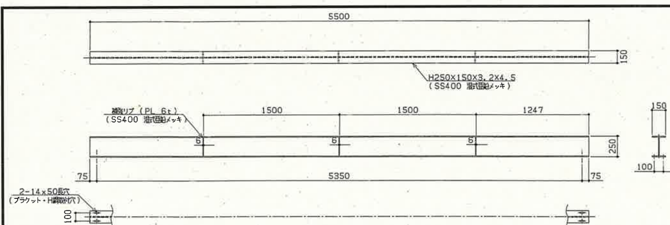
既設受桁①
