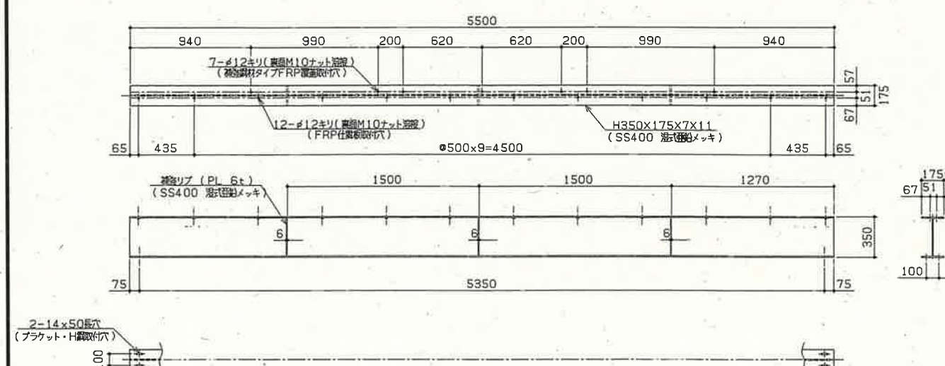
既設受桁③
